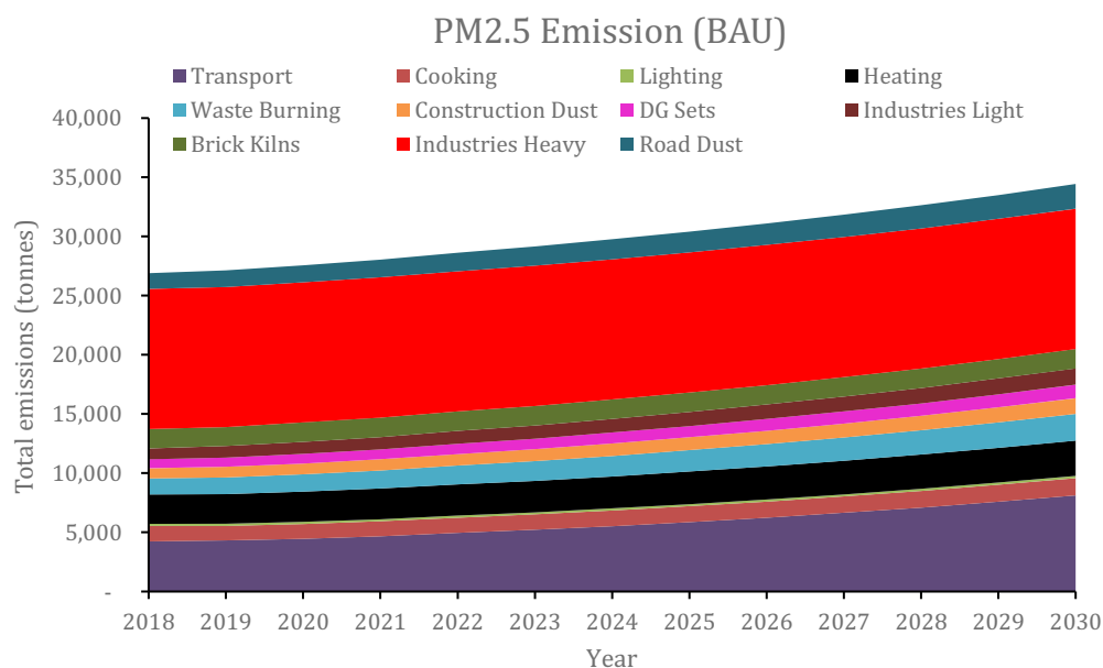
Figure 7 : PM 2.5 emissions (BAU)
